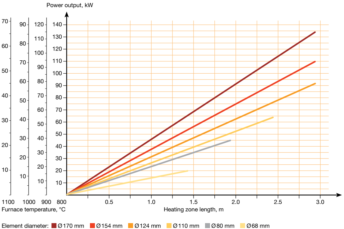
Maximum design power outputs for all standard element diameters at different furnace temperatures
