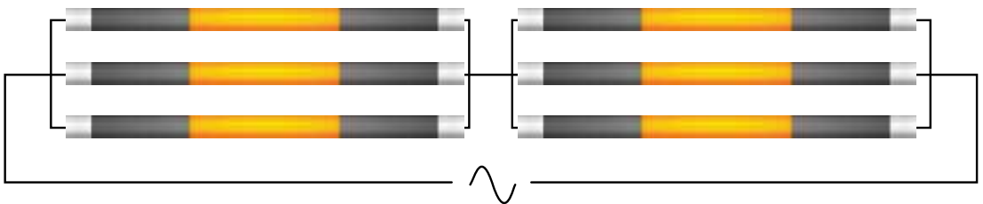
Alternative method of series/parallel connection, not recommended
