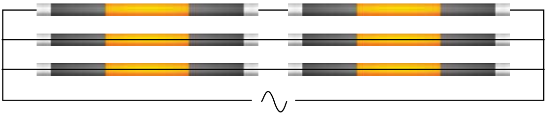
Preferred method of series/parallel connection
